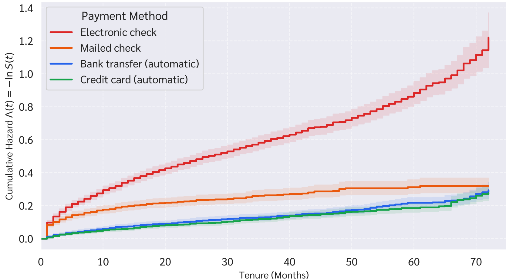
Cumulative Hazard \Lambda(t) by Payment Method
